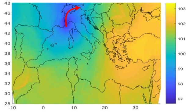
Figure 2 – MSLP field during the October 2018 event and its trajectory.
