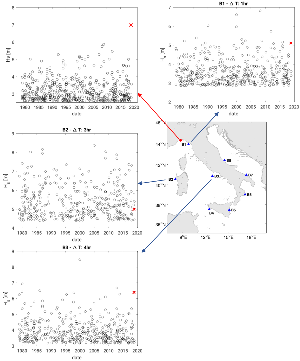
Figure 1 – H_s peak for B1, B2 and B3, extended until December 2018, and peaks at a location in the Gulf of Genoa (not analyzed in the manuscript).
