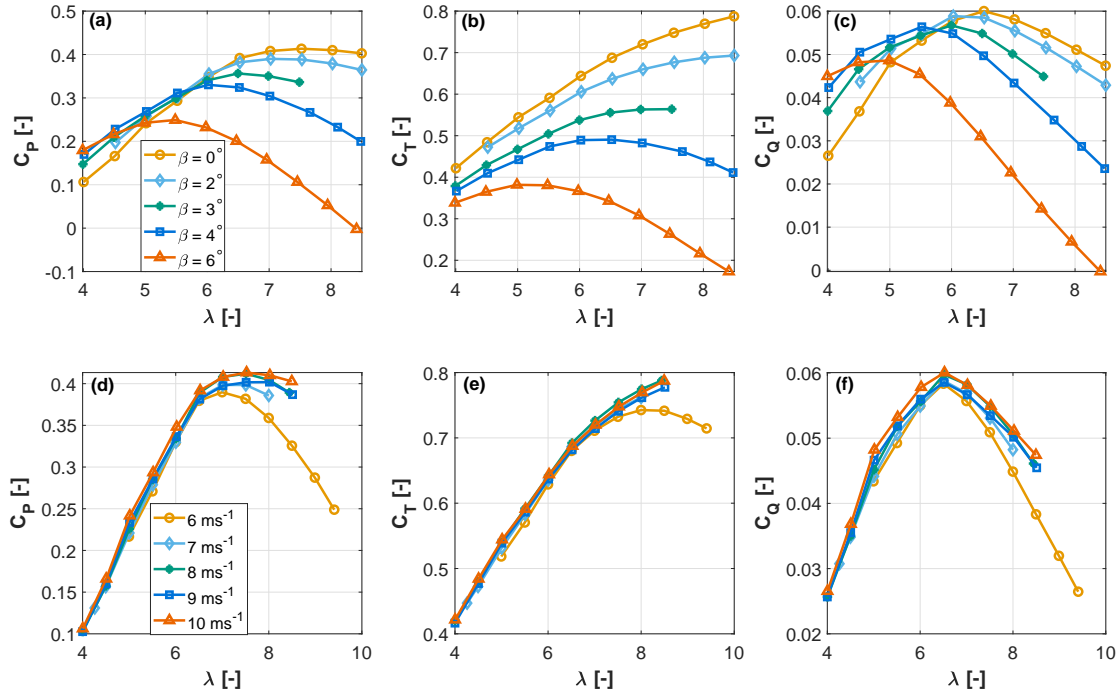
Figure 8. Power C_P (a,d), thrust C_T (b,e) and torque C_Q (c,f) coefficients as functions of TSR \lambda for different pitch angles \beta at 10 ms -1 (a,b,c), and for different wind speeds at the optimum pitch angle \beta = 0^\circ (d,e,f).
