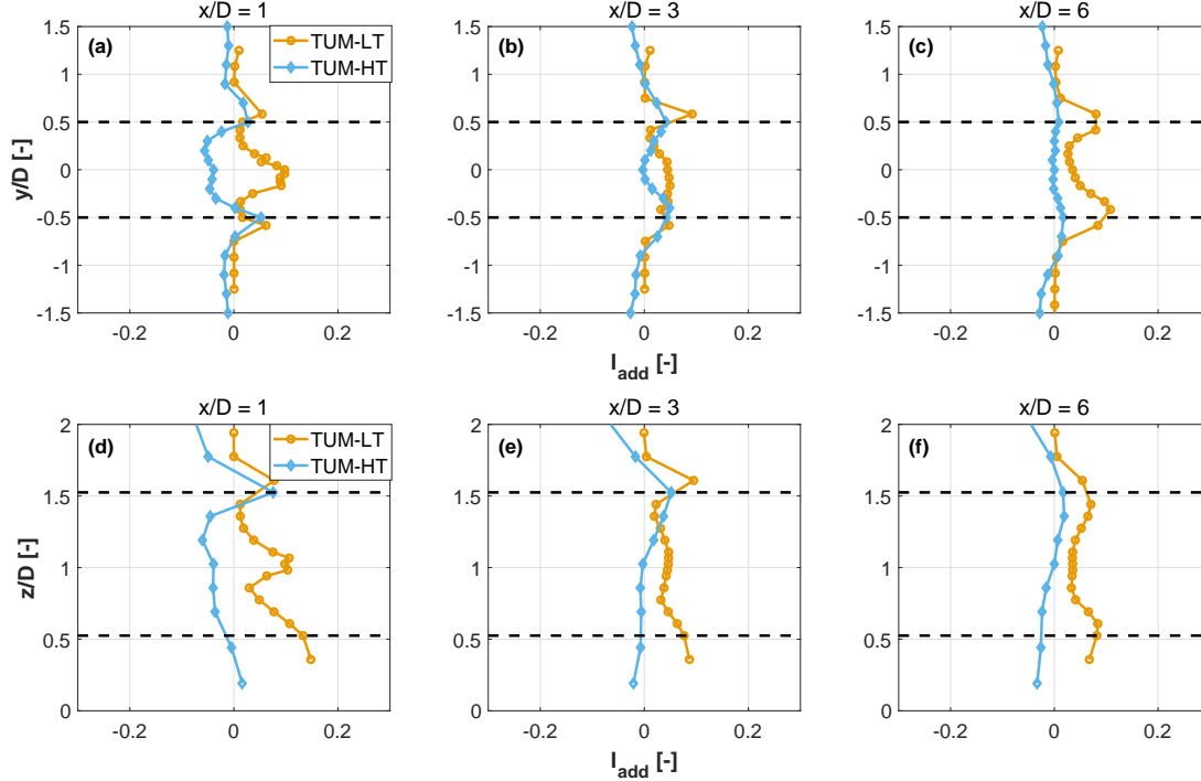
Figure 18. Horizontal (a-c) and vertical (d-f) profiles of added TI at several downstream distances and different inflow conditions. Black dashed lines indicate the rotor tips.
