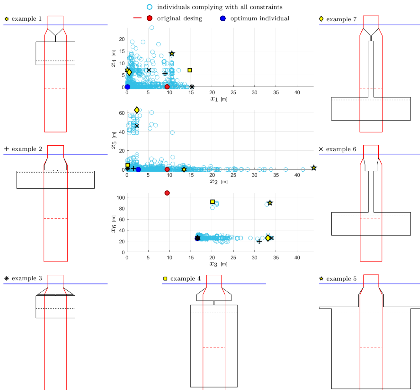
Figure 5. Exemplary potential advanced spar-type floater geometries selected from the individuals complying with all constraints.
