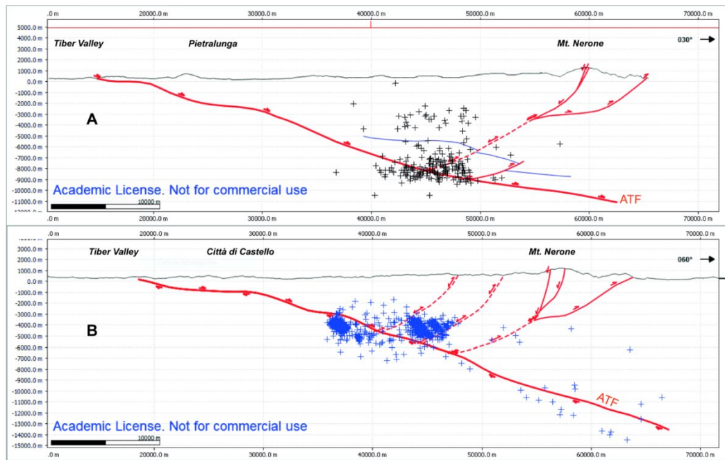
Figure 10: Schematic geological cross-sections showing instrumental earthquakes foci distribution. A section SSW-NNE (redrawn from De Donatis et al., 2020) shows main faults (ATF, thrusts, studied normal faults and negatively inverted thrust ramp; instrumental projected earthquakes from ISIDE Database (ISIDE Working Group, 2007) (black crosses). B section SW-NE (Città di Castello – Monte Nerone) shows also the Marnoso-Arenacea thrusts. Earthquakes from TABOO database (from Valoroso et al., 2017) were projected on the section plane (blue crosses).
