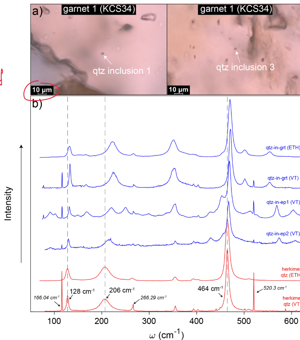
665 Figure 4. Photomicrographs of measured quartz inclusions in garnet from Delfini (a) and Raman spectra of unstrained Herkimer quartz and strained quartz inclusions (b). b) Shown for comparison are Herkimer quartz (red) and quartz inclusion (blue) measurements from Virginia Tech and ETH Zürich. Quartz bands and Ar plasma lines (only VT analyses) are numerically labelled.
