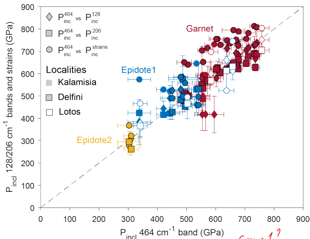
Figure 5. Comparison of P_{inc} determined from different quartz bands using hydrostatic calibrations, and by using phonon-mode Grüneisen tensors (strains). Red, blue, and yellow symbols indicate qtz-in-grt (Group), qtz-in-ep1 (Group 2), and qtz-in-ep2 (Group 3) results, respectively. Diamonds, squares, and circles indicate P_{inc}^{464} vs P_{inc}^{128} , P_{inc}^{464} vs P_{inc}^{206} , and P_{inc}^{464} vs P_{inc}^{strains} results, respectively. No border, filled, and open symbols indicate analyses from Kalamisia, Delfini, and Lotos samples, respectively.
