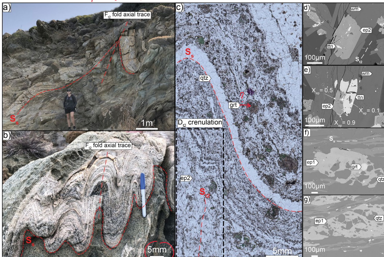
Figure 2. Outcrop, micrograph, and electron images showing stages of retrograde deformation present in southern Delfini. a) Upright folds ( F_2 ) that refold the primary S_1 foliation. b): Core of F_2 folds (below Fig. 2a, KCS34). c): Plane light image of sample KCS34; sample cut perpendicular to the F_2 fold axial plane. Epidotes (ep2) from the upright fold exhibit recrystallization as indicated by alignment with a late S_2 crenulation, and a reduction in inclusions and grain size. d) Ep2 with late titanite (ttn) inclusions. Ep2 is parallel to white mica (wm) that defines S_2 (KCS34). e) Ep2 in textural equilibrium with ttn (KCS34). f) Ep1 parallel to S_1 , with garnet (grt) and quartz (qtz) inclusions that do not define an internal foliation (KCS1621). g) Poikiloblastic ep1 parallel to S_1 , with a weak internal foliation defined by qtz (KCS1621).
