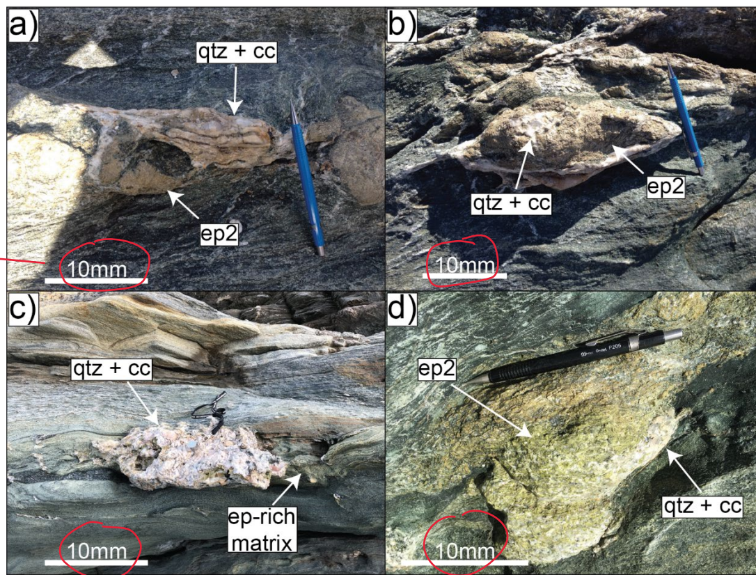
Figure 3. Outcrop photos of epidote boudins sampled for oxygen isotope thermometry. a) SY1613 (Lotos), b) SY1617 (Delfini), c) SY1618 (Delfini), d) SY1623 (Delfini).
