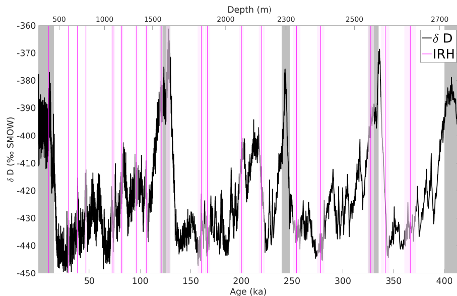
Figure 4. Temporal coverage of the dated IRHs (marked in magenta) over the past four glacial cycles, here displayed on top of \delta D variations measured on the EDC ice core and using the AICC2012 chronology (Bazin et al., 2013). IRH age uncertainties are indicated by pink vertical bounds. Interglacials are highlighted in grey.
