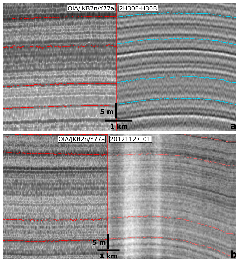
Figure 8. Zoomed-in view of the crossovers and the IRH matches between an OIA transect (OIA/JKB2n/Y77a) and (a) DELORES transect 2H30E-H30B, and (b) MCoRDS transect 20121127_01. Vertical and horizontal scales are provided on each panel.
