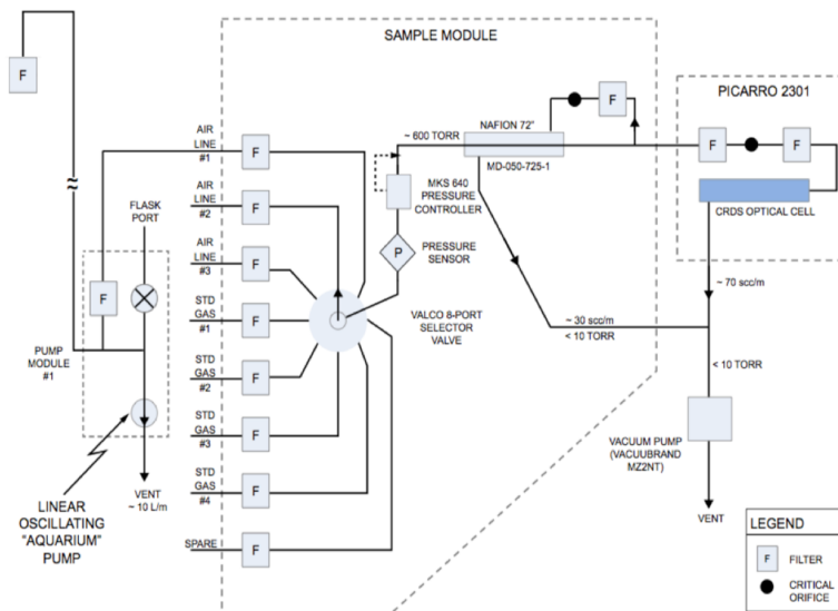
185 Figure 4. Plumbing diagram for the Earth Networks sampling system implemented at the NEC tower stations. Figure replicated from Fig. S1 in Verhulst et al. (2017), adapted from Welp et al. (2013).
