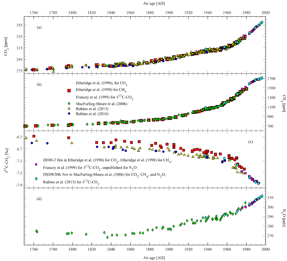
Figure 23: Published and unpublished Industrial Period (1750-2000 AD) GHG records from Law Dome ice and firn, extracted and measured at CSIRO ICELAB-GASLAB. (a) \text{CO}_2 ; (b) \text{CH}_4 ; (c) \delta^{13}\text{C}-\text{CO}_2 and (d) \text{N}_2\text{O}
