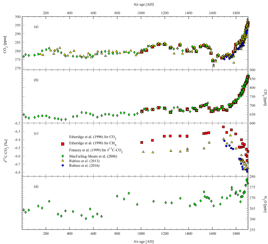
85 Figure 42: Published Pre-Industrial Period (1-1900 AD) GHG records from Law Dome ice extracted and measured at CSIRO ICELAB-GASLAB. (a) CO 2 ; (b) CH 4 ; (c) δ 13 C-CO 2 and (d) N 2 O
