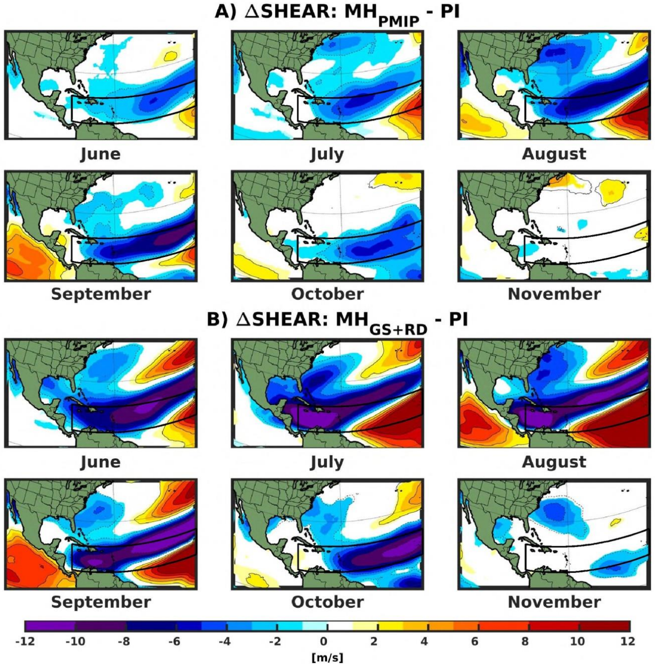
Figure A12: Monthly mean changes in climatological wind shear (200 hPa – 850hPa) for (A) MH_{PMIP} and (B) MH_{GS+RD} relative to PI. The black box shows the approximate present-day Main Development Region (MDR). Only values that are significantly different at the 5% level using a local (grid-point) t test are shaded. The contour lines follow the colorbar scale (dashed, negative anomalies; solid, positive anomalies); the 0 line is omitted for clarity.
