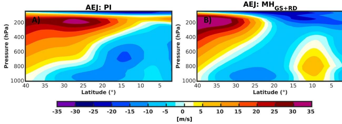
Figure 8: African Easterly Jet (AEJ) represented through a vertical cross section of zonal mean (0-40°N; 20°W-30°W) seasonal climatological zonal winds for (A) PI and (B) MH GS+RD experiments, respectively.
