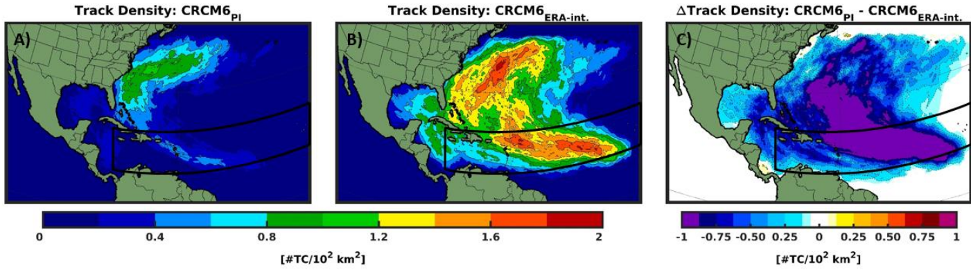
Figure A2: Climatological track density (JJASON) for (A) pre-industrial experiment and (B) ERA-Interim driven experiment. (C) Changes in track density between the two simulations. The black box shows the approximate present-day Main Development Region (MDR). Only values that are significantly different at the 5% level using a local (grid-point) t test are shaded. The contour lines follow the colorbar scale (dashed, negative anomalies; solid, positive anomalies); the 0 line is omitted for clarity.
