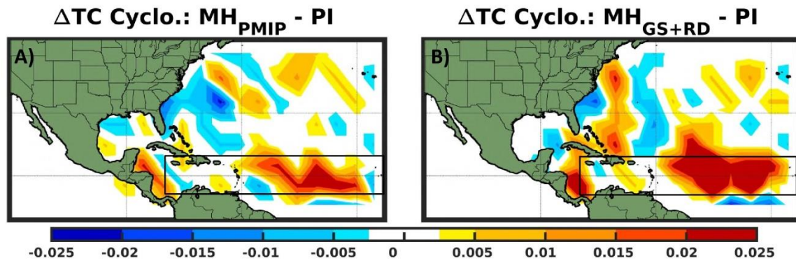
Figure 4: TC seasonal (June to November) cyclogenesis density anomaly for (A) \text{MH}_{\text{PMIP}} and (B) \text{MH}_{\text{GS+RD}} experiments relative to PI represented over a 5° meshgrid Mercator projection. The black box shows the approximate present-day main development region (MDR).
