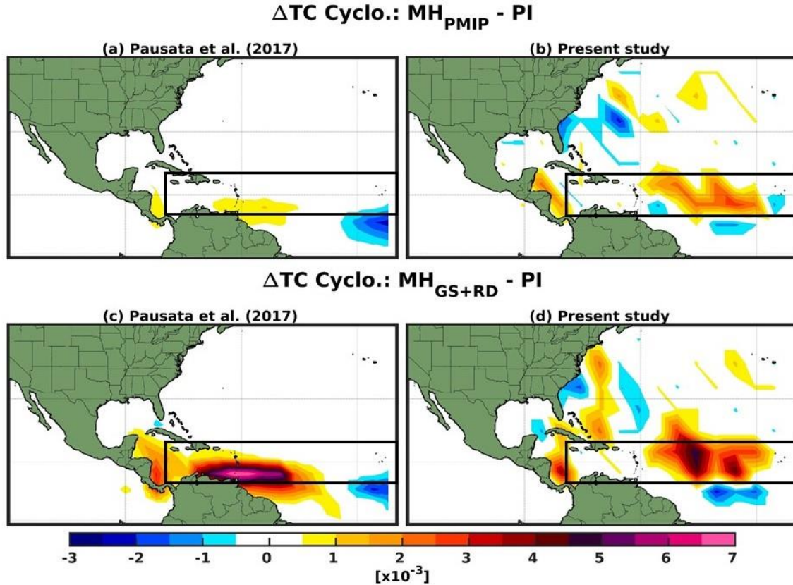
Figure A10: Comparison between TC seasonal cyclogenesis density anomalies for (a – b) MH_{PMIP} and (c – d) MH_{GS+RD} relative to PI between (a – c) Pausata et al. (2017) and (b – d) the present study. Note that data are represented over a 5^\circ meshgrid Mercator projection in the present study while in Pausata et al. (2017) a 4^\circ meshgrid is used to represent the fields. The black box shows the approximate present-day main development region (MDR).
