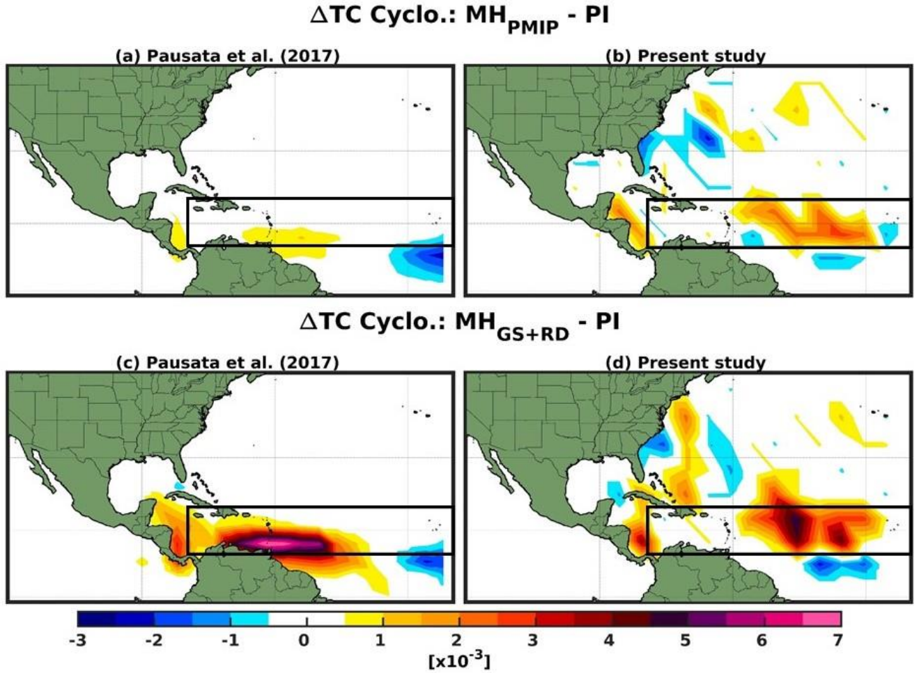
Figure A10: Comparison between TC seasonal cyclogenesis density anomalies for (a – b) \text{MH}_{\text{PMIP}} and (c – d) \text{MH}_{\text{GS+RD}} relative to PI between (a – c) Pausata et al. (2017) and (b – d) the present study. Note that data are represented over a 5^\circ meshgrid Mercator projection in the present study while in Pausata et al. (2017) a 4^\circ meshgrid is used to represent the fields. The black box shows the approximate present-day main development region (MDR).
