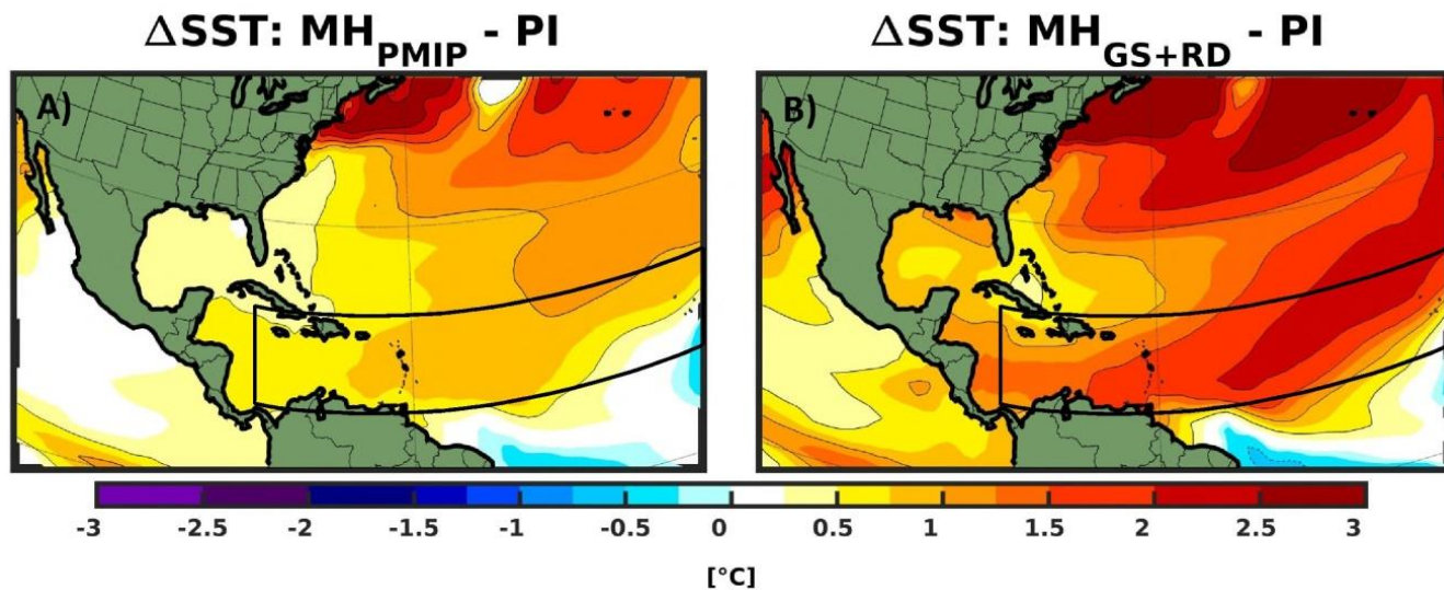
Figure A6: Climatological (JJASON) changes in Sea Surface Temperature (SST) for (A) \text{MH}_{\text{PMIP}} and (B) \text{MH}_{\text{GS+RD}} experiments relative to PI. The black box shows the approximate present-day Main Development Region (MDR). Only values that are significantly different at the 5% level using a local (grid-point) t test are shaded. The contour lines follow the colorbar scale (dashed, negative anomalies; solid, positive anomalies); the 0 line is omitted for clarity.
