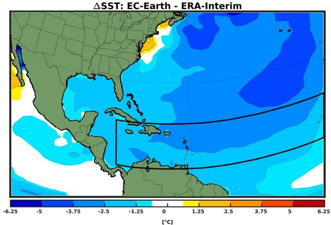
Figure A3: Climatological changes in Sea Surface Temperature (SST) between simulated EC-Earth preindustrial climate and ERA-Interim reanalysis from 1979 to 2008. The black box shows the approximate present-day main development region (MDR). The contour lines follow the colorbar scale (dashed, negative anomalies; solid, positive anomalies); the 0 line is omitted for clarity.
