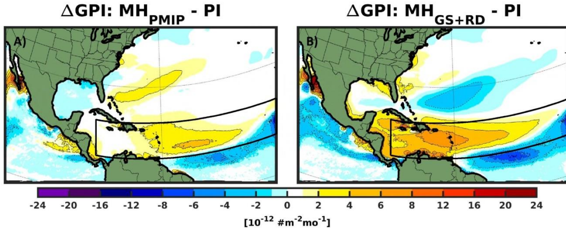
Figure 3: Changes in seasonal Genesis Potential Index - GPI (June to November, JJASON) for (A) \text{MH}_{\text{PMIP}} and (B) \text{MH}_{\text{GS+RD}} experiments relative to PI. The black box shows the approximate present-day main development region (MDR). Only values that are significantly different at the 5% level using a local (grid-point) t test are shaded. The contour lines follow the colorbar scale (dashed, negative anomalies; solid, positive anomalies); the 0 line is omitted for clarity.
