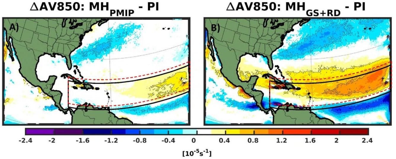
Figure A5: Climatological (June to November, JJASON) changes in 850 hPa absolute vorticity relative to PI for (A) MH_{PMIP} experiment and (B) MH_{GS+RD} experiment. The black box represents the approximate present-day MDR. Red dotted box shows the approximate shift in the absolute vorticity maxima. Only values that are significantly different at the 5% level using a local (grid-point) t test are shaded. The contour lines follow the colorbar scale (dashed, negative anomalies; solid, positive anomalies); the 0 line is omitted for clarity.
