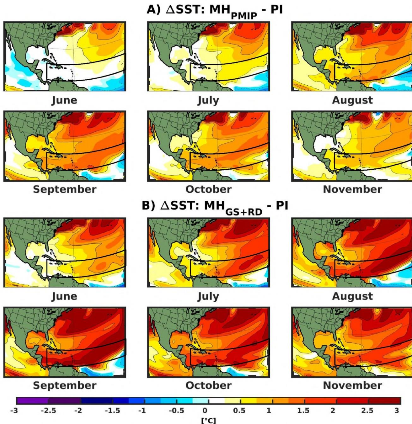
Figure A11: Monthly mean changes in climatological Sea Surface Temperature (SSTs) for (A) \text{MH}_{\text{PMIP}} and (B) \text{MH}_{\text{GS+RD}} relative to PI experiment. The black box shows the approximate present-day Main Development Region (MDR). Only values that are significantly different at the 5% level using a local (grid-point) t test are shaded. The contour lines follow the colorbar scale (dashed, negative anomalies; solid, positive anomalies); the 0 line is omitted for clarity.
