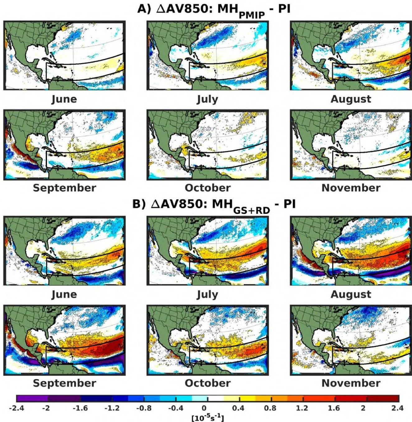
Figure A13: Monthly mean changes in 850 hPa absolute vorticity for (A) MH_{PMIP} and (B) MH_{GS+RD} relative to PI. The black box shows the approximate present-day Main Development Region (MDR). Only values that are significantly different at the 5% level using a local (grid-point) t test are shaded. The contour lines follow the colorbar scale (dashed, negative anomalies; solid, positive anomalies); the 0 line is omitted for clarity.
