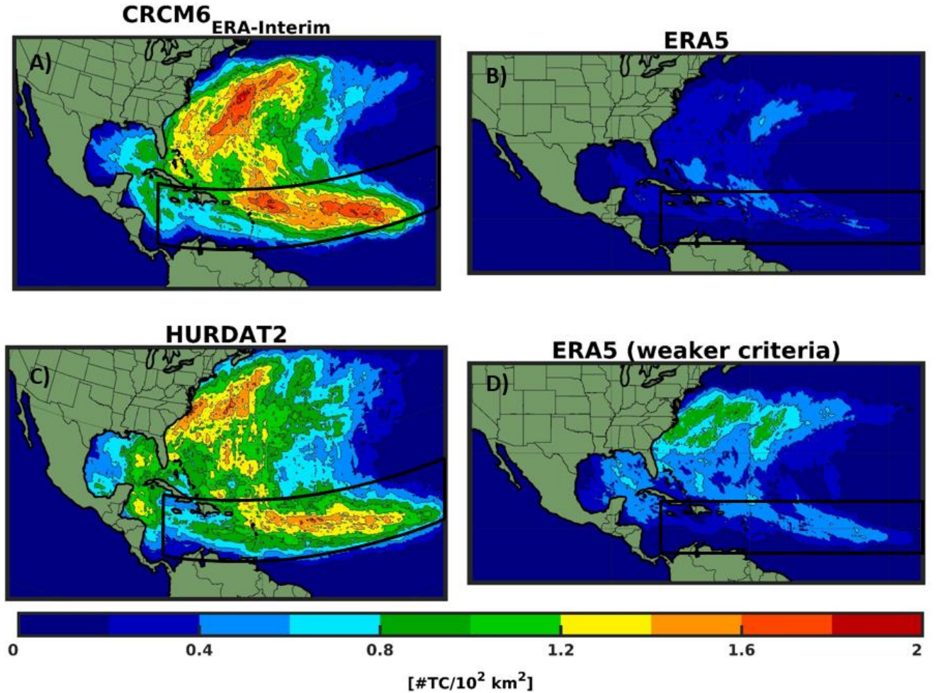
Figure A1: June to November (JJASON) climatology (1980-2009) of (A) track density for the CRCM6 ERA-Interim driven experiment at 0.22^\circ ; (B) ERA5 reanalysis data at 0.25^\circ ; (C) Observed TCs from the HURDAT data base at 0.11^\circ and (D) ERA5 reanalysis data using weaker detection criteria at 0.25^\circ . The black box shows the present-day Main Development Region (MDR). Note that the ERA5 figures are projected over a Mercator grid while the other two figures use the Equidistant Cylindrical Projection. The contour lines follow the colorbar scale.
