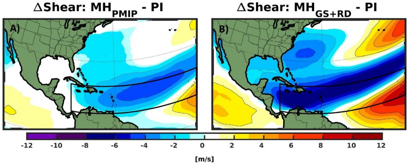
Figure A7: Changes in vertical wind shear (300 hPa – 850 hPa) for (A) \text{MH}_{\text{PMIP}} and (B) \text{MH}_{\text{GS+RD}} experiments relative to PI. The black box shows the approximate present-day Main Development Region (MDR). Only values that are significantly different at the 5% level using a local (grid-point) t test are shaded. The contour lines follow the colorbar scale (dashed, negative anomalies; solid, positive anomalies); the 0 line is omitted for clarity.
