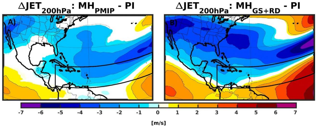
Figure A9: Climatological (JJASON) changes in 200 hPa wind speed for (A) \text{MH}_{\text{PMIP}} and (B) \text{MH}_{\text{GS+RD}} experiments relative to PI. The black box shows the approximate present-day Main Development Region (MDR). Only values that are significantly different at the 5% level using a local (grid-point) t test are shaded. The contour lines follow the colorbar scale (dashed, negative anomalies; solid, positive anomalies); the 0 line is omitted for clarity.
