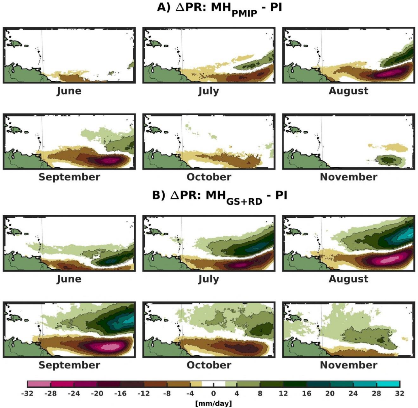
Figure A4: Monthly mean climatological changes in precipitation for (A) MH_{PMIP} and (B) MH_{GS+RD} relative to PI in the domain 23^{\circ} \text{ W} - 75^{\circ} \text{ W} , 5^{\circ} \text{ N} - 23^{\circ} \text{ N} . Only values that are significantly different at the 5% level using a local (grid-point) t test are shaded. The contour lines follow the colorbar scale (dashed, negative anomalies; solid, positive anomalies). The 0 line is omitted for clarity.
