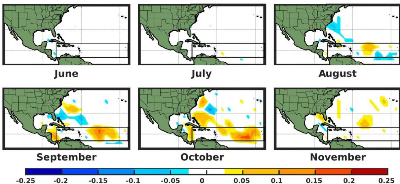
Figure A14: TC seasonal (June to November) cyclogenesis density anomaly for (A) MH_{PMIP} and (B) MH_{GS+RD} experiments relative to PI represented over a 5° meshgrid Mercator projection. The black box shows the approximate present-day Main Development Region (MDR).
