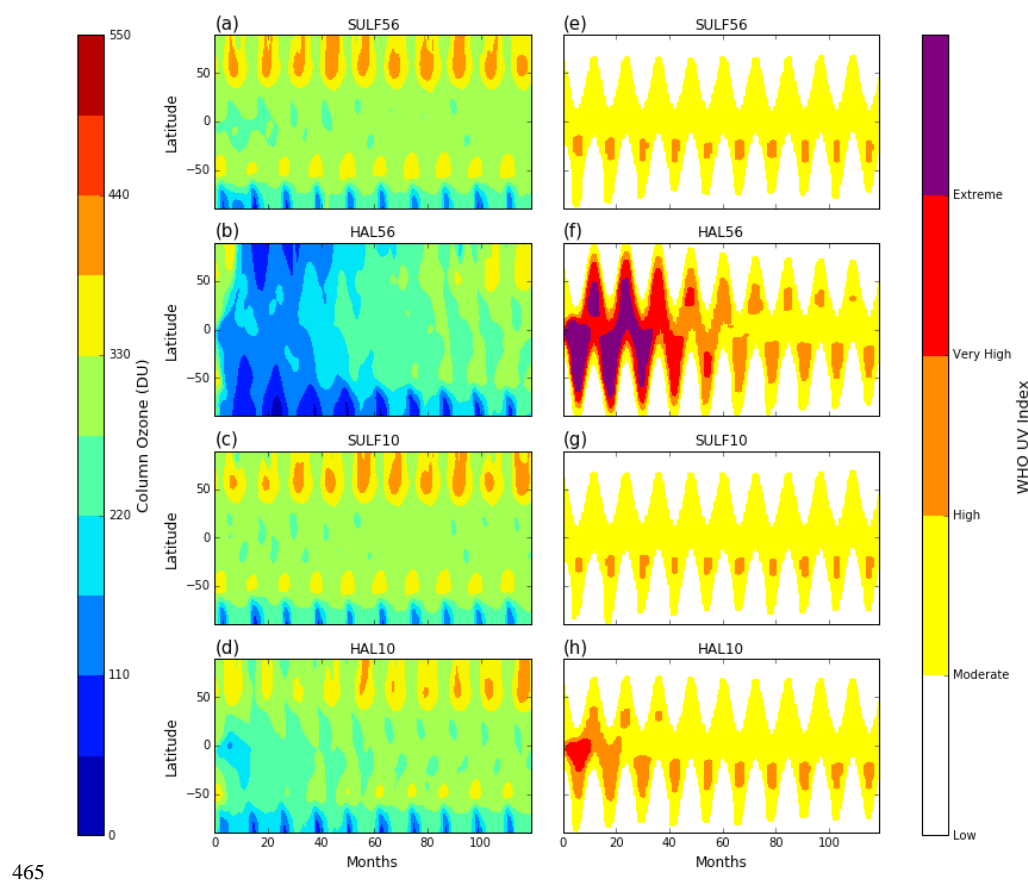
Figure 12 Zonal mean column ozone (a) SULF56, (b) HAL56, (c) SULF10, (d) HAL10. Ozone hole conditions are simulated when the column ozone < 220 DU. Zonal mean surface UV exposure due to column ozone change (WHO UV Index) (e) SULF56, (f) HAL56, (g) SULF10, (h) HAL10.
