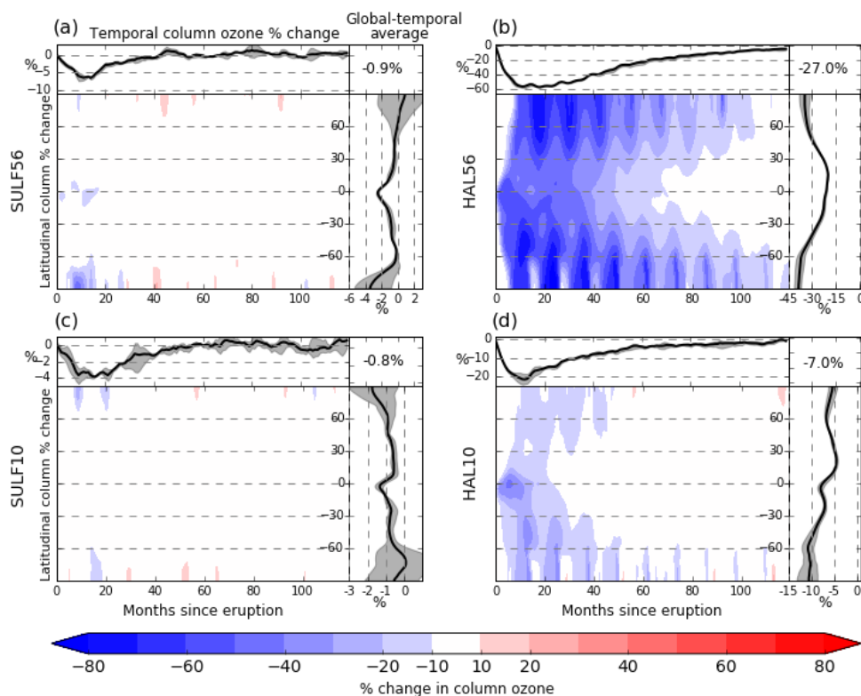
Figure 5 Ozone% difference in response to the simulated volcanic eruptions (a) SULF56, (b) HAL56, (c) SULF10, (d) HAL10. Global averages of total column ozone perturbation are traced atop each panel as a function of time. Temporal average ozone anomalies are traced right, note different scales. Global-temporal averages are enumerated in the top right. Red colors indicate column ozone enhancement, and blue colors indicate column 330 ozone depletion.
