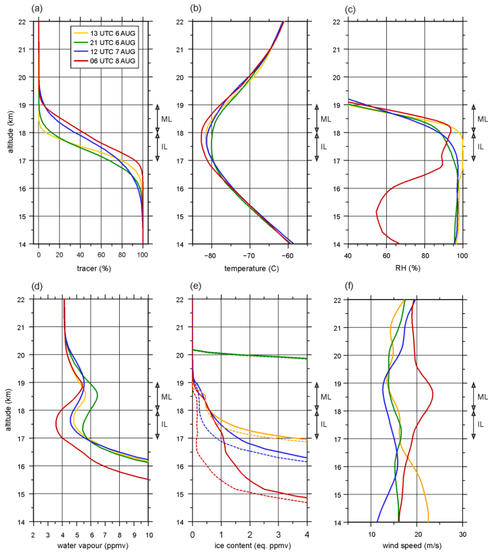
Figure 11. Vertical profiles of (a) tracer (%), (b) temperature ( ^\circ\text{C} ), (c) relative humidity (%), mixing ratios of (d) water vapour (ppmv), (e) ice content (eq. ppmv), and (f) wind speed ( \text{m s}^{-1} ) across the hydration patch along the trajectory at 13:00 UTC (yellow line), 21:00 UTC (green line) on 6 August, 12:00 UTC on 7 August (blue line), and 06:00 UTC (red
