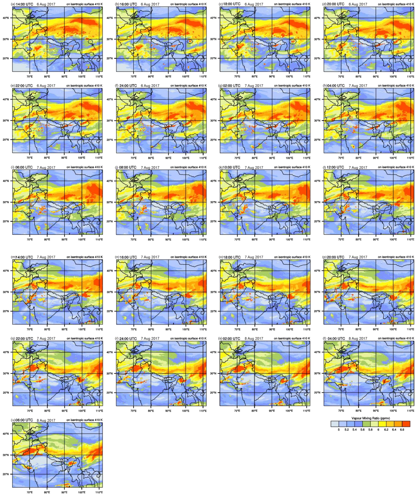
Figure A. Horizontal distributions of water vapour at 410 K isentropic altitude every 2 hour from 14:00 UTC on 6 August to 06:00 UTC on 8 August 2017. The target hydration patch is marked by an ellipse with dashed line.
