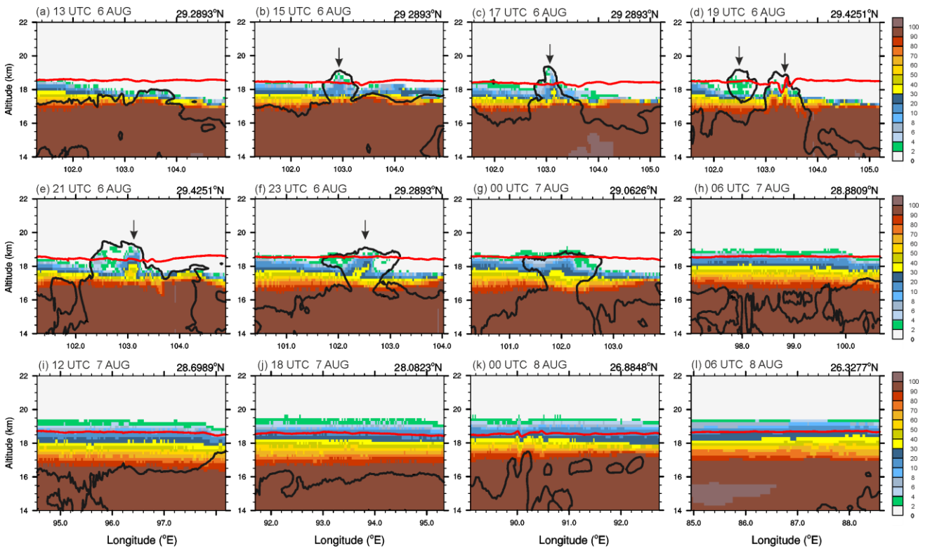
Figure 8. Same as Fig. 7 but for the tracer (%). The isentropic altitude of 410 K is depicted by the red line. The changes of the tropospheric tracer by convective overshoots is marked by downward arrows.
