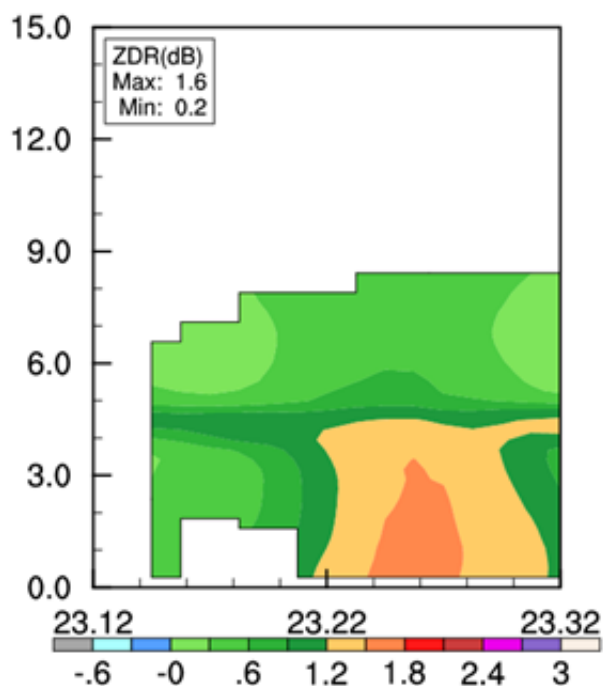
Fig. R1 Temporal-averaged vertical cross-section along C-D in Fig. 6 of the simulated differential reflectivity (dB, shadings) during the period from 0600 BST to 0700 BST 7 May, 2017.
