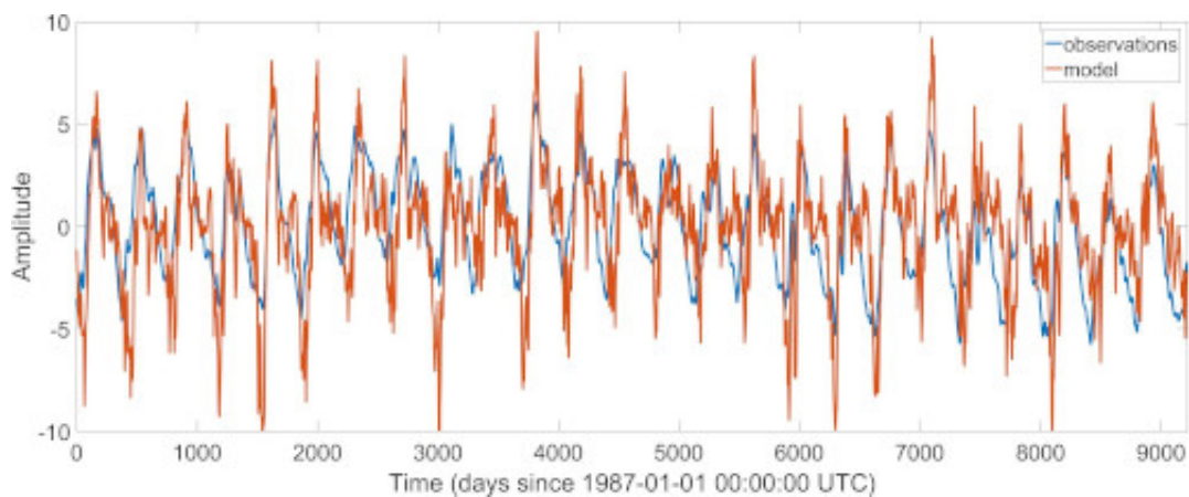
Figure R1: Time variations of the amplitude of EOF1 for both observation and model.
