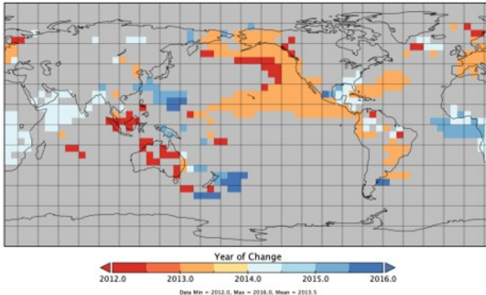
Surface Temperatures Year Of Change – 5 Year Summary NCDC/PSL After 1950, P \leq 0.05
