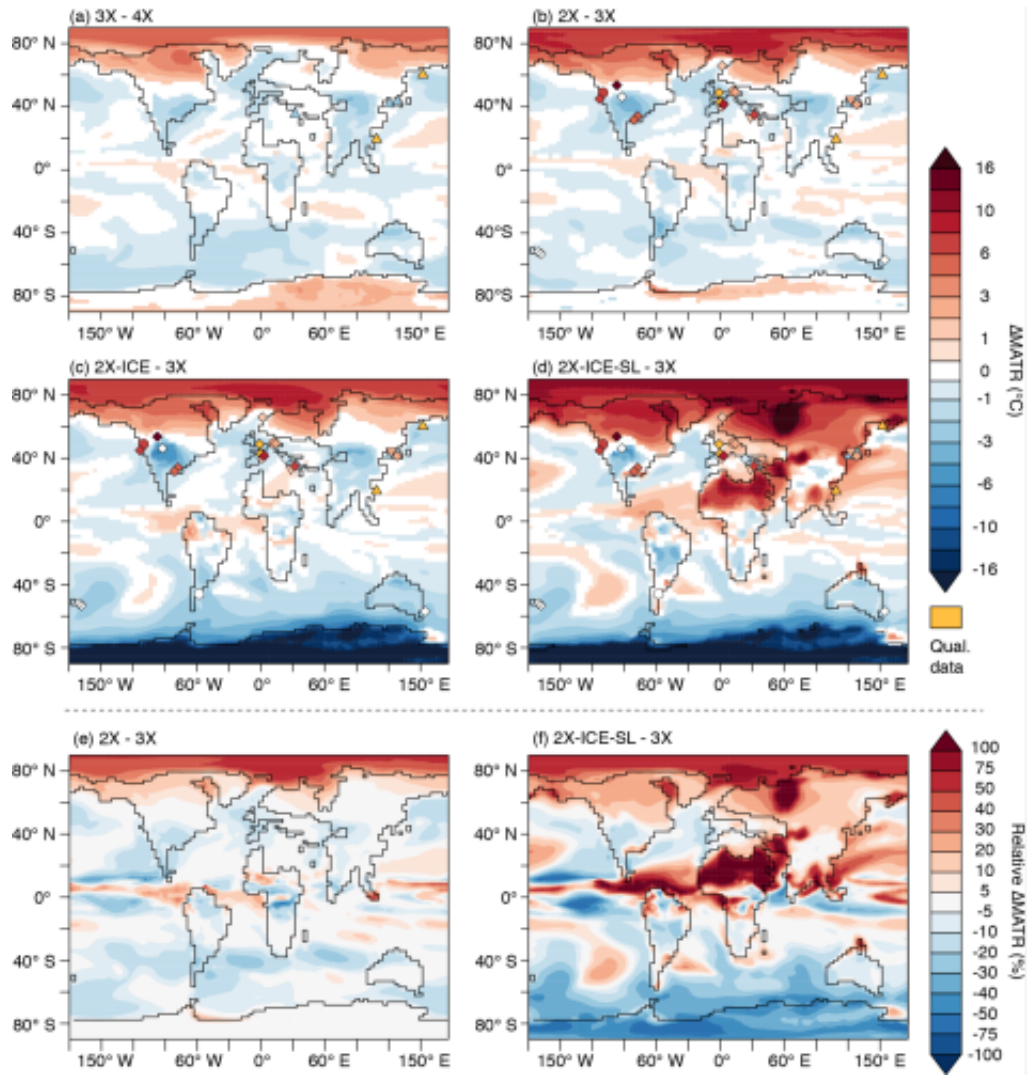
Revised Figure 4 - Subfigures e,f now indicate relative \Delta MATR, for 2X-3X and 2X-ICE-SL - 3X respectively (%).
