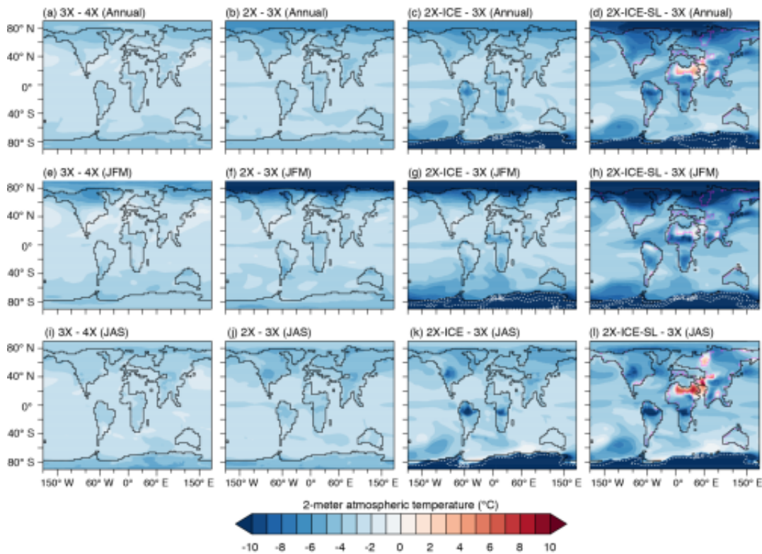
Revised Figure 2 - After modification of subfigures d,h,l. Shorelines are visible in magenta.
