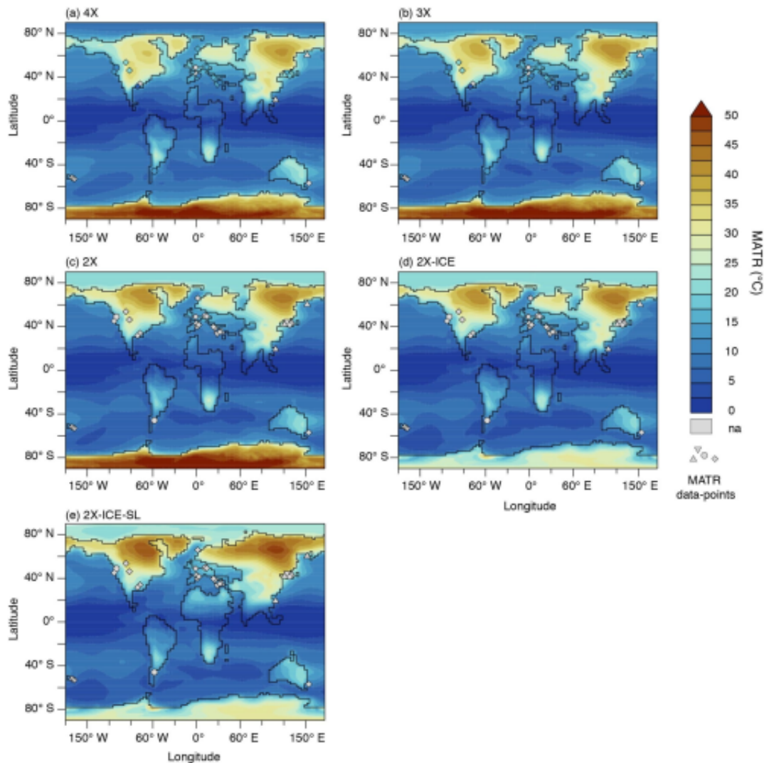
Revised Figure S2 with Eocene MATR values on subfigures a,b.
