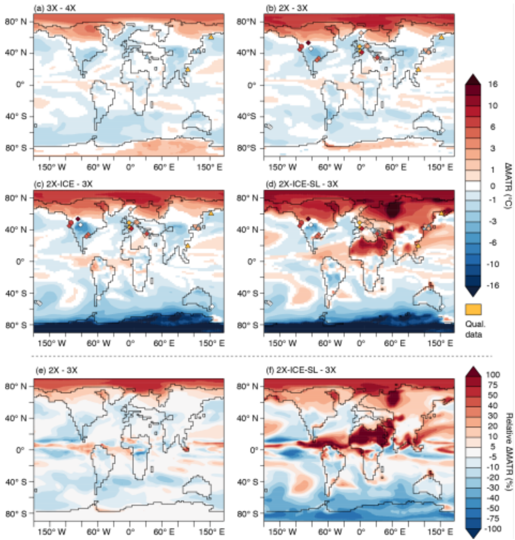
Revised Figure 4 - Subfigures e,f now indicate relative \Delta\text{MATR} , for 2X-3X and 2X-ICE-SL - 3X respectively (%).
