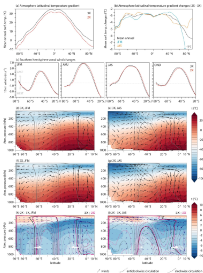
New Figure S4 - Changes in atmospheric temperature and vertical circulation patterns between 3X and 2X in the Southern Hemisphere. (a,b) latitudinal surface temperature gradient; (c) zonal winds; (d-g) Air temperature (shaded), atmospheric cell extent (zonal mean streamfunction, lines) and vertical winds (arrows) in austral summer and winter for 3X and 2X
