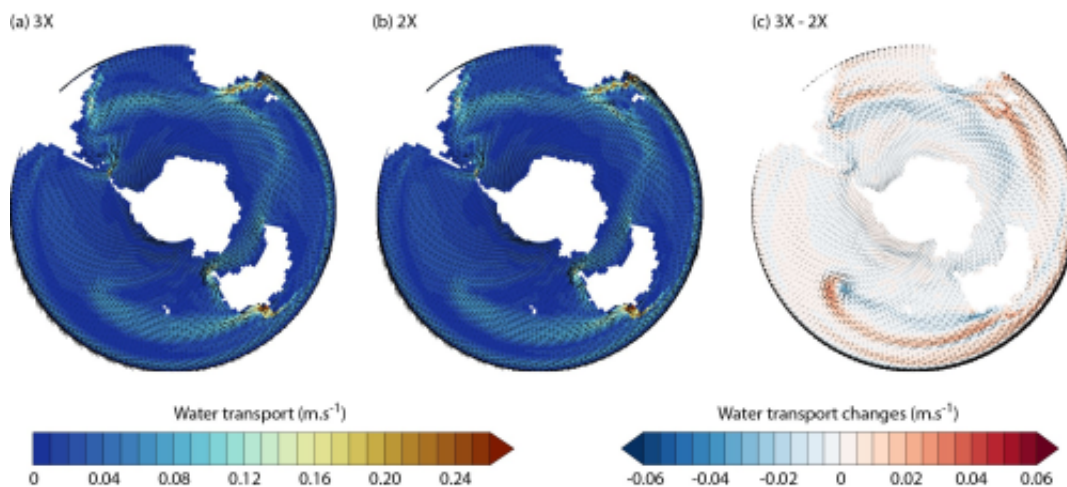
New Figure S5 - Annually 0–300 m depth averaged current velocity through the Southern Ocean (annual average, m.s-1).
