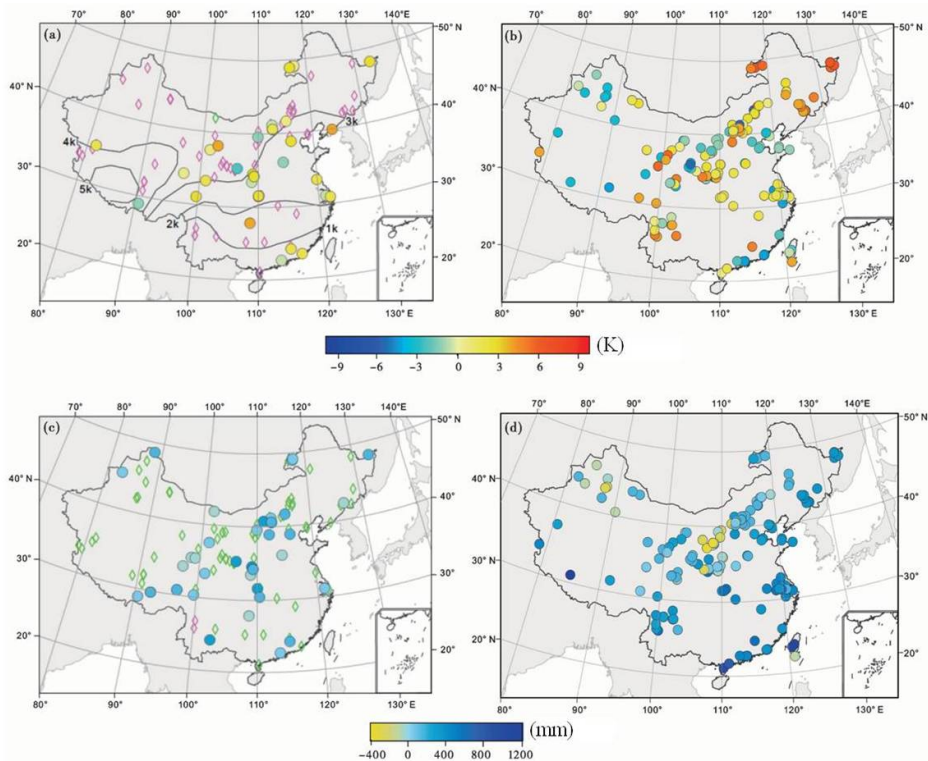
Figure 1. Comparison between our climate reconstruction and previous reconstruction. (a) Previous temperature results. Diamond is the qualitative reconstruction, red is the temperature increase and green is the temperature decrease; Circle is quantitative reconstruction; (b) Mean annual temperature reconstruction in this study; (c) Previous precipitation results, diamond is the qualitative reconstruction, red is the precipitation increase and green is the precipitation decrease; Circle is quantitative reconstruction; (d) Mean annual precipitation reconstruction in this study.
