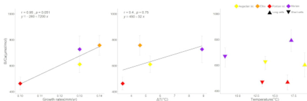
Figure 11: Correlation plots of growth rates and seawater temperature with B/Ca in L. corallioides samples analysed in this study. Spearman's coefficient r , the p-value and the line equation are given. Temperature variations ( \Delta T ) correspond to the differences between the maximum and minimum temperature registered over 11 years of monthly reanalysis (ORAS5). The B/Ca means measured in long and short cells correspond respectively to the maximum and minimum temperature.
