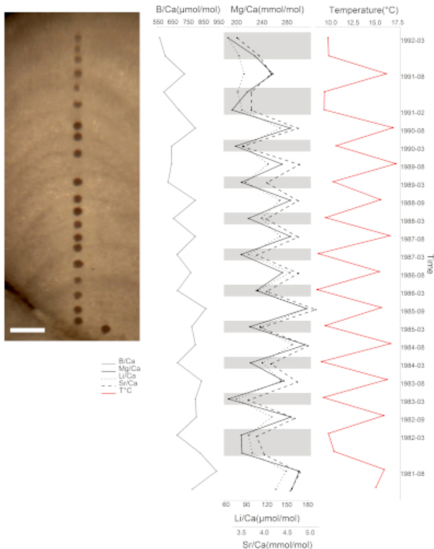
Figure 12 (new): Elements ratio of L. corallioides collected in Morlaix Bay (scale bar = 200 \mu\text{m} ). Mg, Li and Sr/Ca show cyclic variations the same as the local seawater temperature. In the timeline, the coldest and the warmest months have been reported, which correspond to dark and light bands of growth. Elements/Ca in the missing bands have been calculated as the means of the values measured in warm or cold periods. Monthly means of temperature have been extracted by ORAS5 reanalysis.
