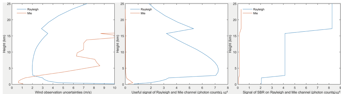
Fig. 1. Comparisons between the wind observations of Rayleigh channel and Mie channel. (a) Wind observation uncertainties; (b) useful signal of atmospheric backscatter; (c) signal excited by SBR.
