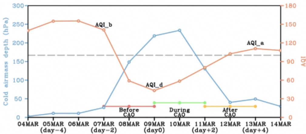
Figure R3. Time series of the regional averaged cold airmass depth (blue line) and AQI (orange line) in northern and eastern China (114°–122°E, 30°–40°N). The gray dashed line denotes the threshold value of the cold airmass depth.
