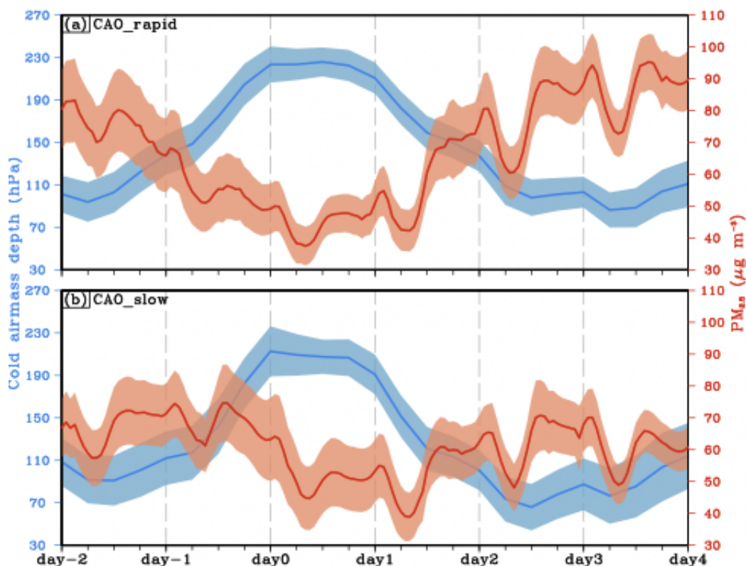
Figure R2. Evolutions of spatial averaged (northern and eastern China: 114°–122°E, 30°–40°N) cold airmass depth and PM 2.5 concentration during CAOs. (a) and (b) are composited by the CAO_rapid events and CAO_slow events, respectively. Shading represents the 95% confidence interval of the composited mean value.
