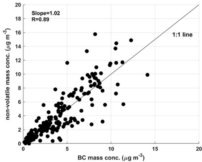
Figure R1. Black carbon (BC) mass concentration measured by AE-33 vs. the non-volatile mass concentration estimated from the VTDMA for winter 2019 periods. Estimation of the non-volatile mass concentration was made assuming a density of 1.6 \text{ g cm}^{-3} .
