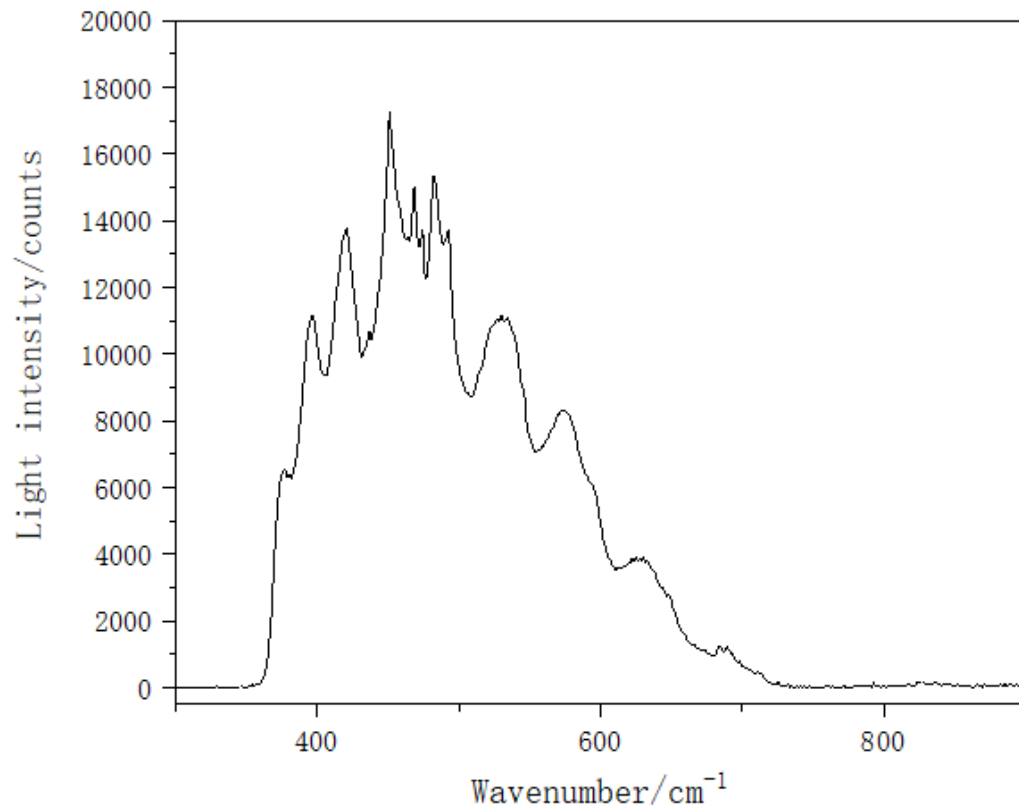
Fig. 1. The spectrum of the Xe lamp coupled with an optical fiber (model CEL-TCX250).
