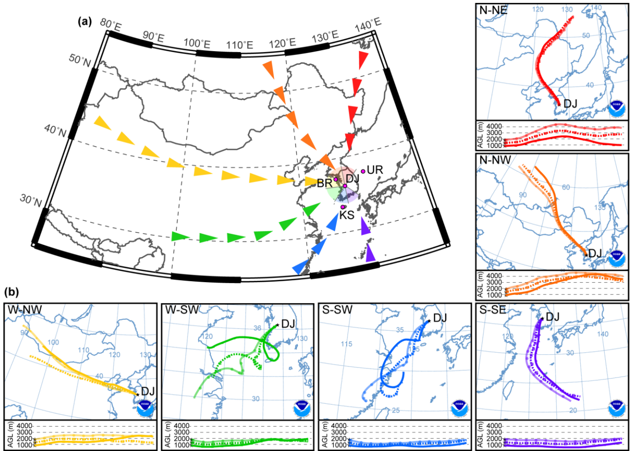
Figure 1: Figure 1: (a) Schematic diagram of dust transport path, BR: Baekryeongdo, DJ: Daejeon, KS: Kosan, UR: Ulreongdo. (b) Representative examples of HYSPLIT backward trajectories ending at DJ. Trajectories of dust transport at 1000 m, 1500 m, and 2000 m above mean sea level (AMSL) were traced for 72 hours. ADS was classified into six transport path on the basis of wind azimuth during the first 24 hours of each ADS event as N-NE (northerly 0° to northeasterly 45°), N-NW (northerly 360° to northwesterly 315°), W-NW (westerly 270° to northwesterly 315°), W-SW (westerly 270° to southwesterly 235°), S-SW (southerly 180° to southwesterly 235°), and S-SE (southerly 180° to southeasterly 135°).
