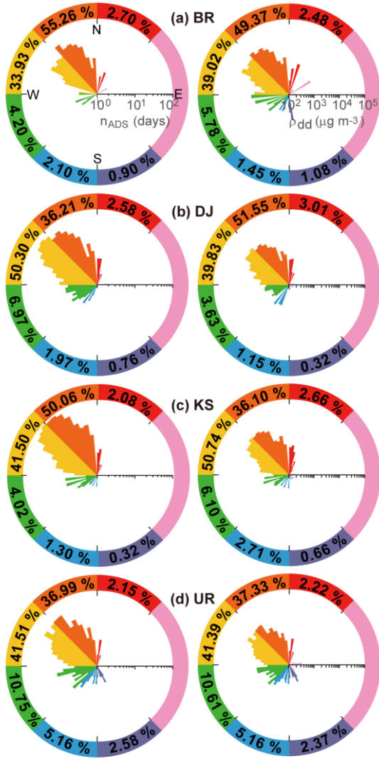
Figure 7: Spatial distribution of ADS on a Rose diagram for (a) BR, (b) DJ, (c) KS, (d) UR. The left panel shows an angular distribution of number of days each year with ADS events ( n_{\text{ADS}} ). The right panel shows an angular distribution of dust densities ( \rho_{\text{dd}} ).
