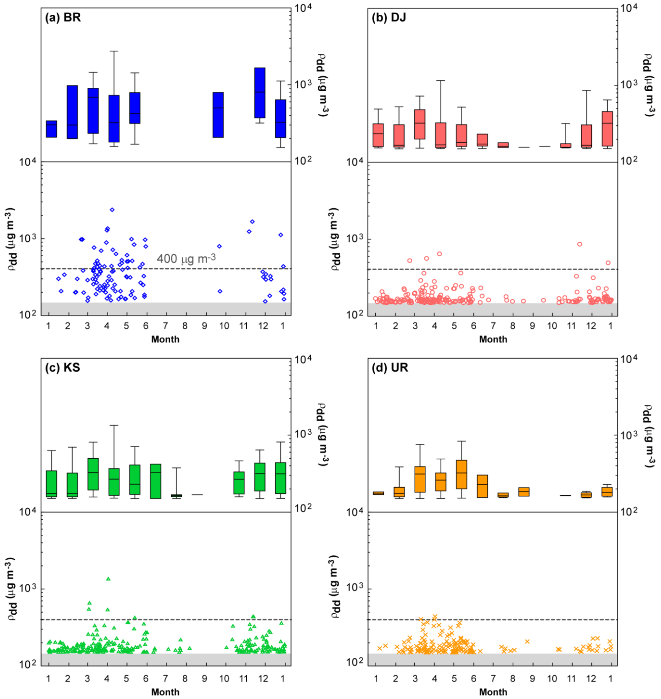
Figure 5: Monthly variations of dust density ( \rho_{dd} ) at (a) BR, (b) DJ, (c) KS, (d) UR. The lower panel shows a distribution of individual dust density. Data symbols and reference lines are as in Fig. 4.
