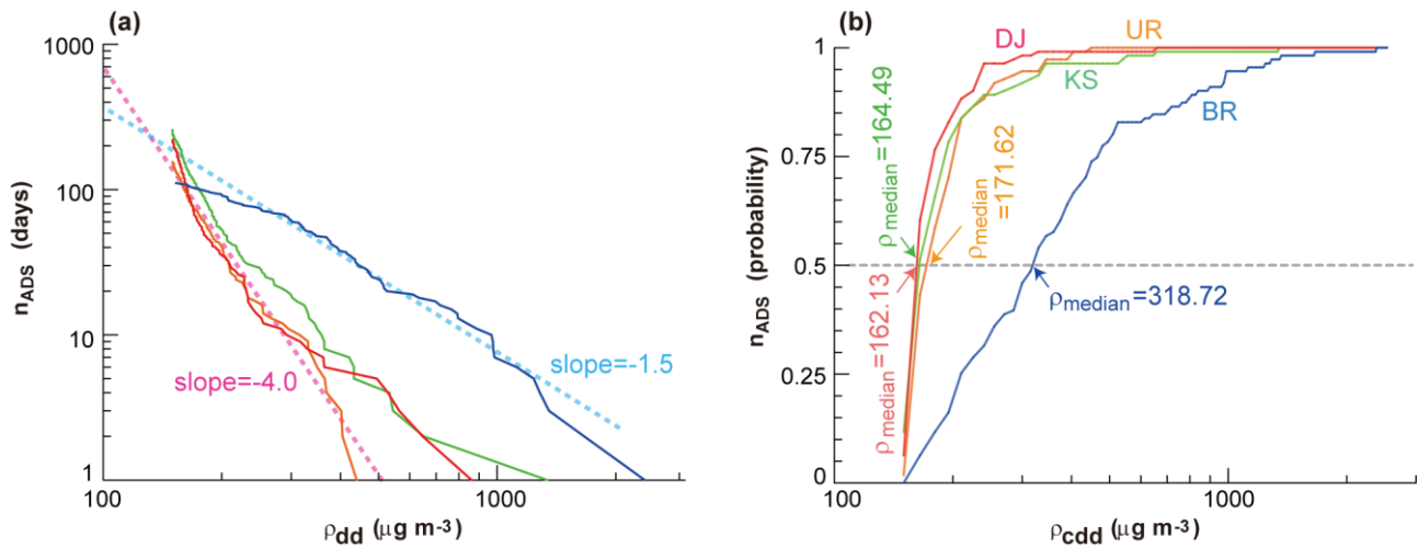
Figure 6: (a) Power-law fit to the ADS events as a function of dust density ( \rho_{\text{dd}} ). The two reference lines are (n_{\text{ADS}}) \propto (\rho_{\text{dd}})^{-1.5} and (n_{\text{ADS}}) \propto (\rho_{\text{dd}})^{-4.0} . (b) Cumulative distribution functions for the ADS data. Median values of dust densities ( \rho_{\text{median}} ) were 318.72 \mu\text{g m}^{-3} for BR, 162.13 \mu\text{g m}^{-3} for DJ, 164.49 \mu\text{g m}^{-3} for KS, and 171.62 \mu\text{g m}^{-3} for UR.
