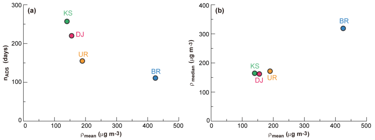
Figure 8: (a) An inverse correlation between ( n_{\text{ADS}} ) and annual mean dust densities ( \rho_{\text{mean}} ). (b) A positive correlation between median dust densities ( \rho_{\text{median}} ) and annual mean dust densities ( \rho_{\text{mean}} ).
