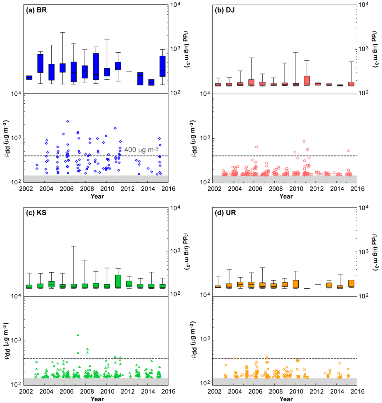
Figure 4: Annual variations of dust density ( \rho_{dd} ) at (a) BR, (b) DJ, (c) KS, (d) UR. The lower panel shows a distribution of individual dust density. The upper panel displays boxplots where central box represents the inter-quartile of annual mean dust density and whisker lines are extending beyond the maximum and the minimum. In the present study, individual ADS event was accounted as the day with advisory warning with ( \rho_{dd} ) exceeds 150 \mu\text{g m}^{-3} for an hour. Another reference line for more significant danger warning with ( \rho_{dd} ) exceeds 400 \mu\text{g m}^{-3} for an hour was marked for comparison.
