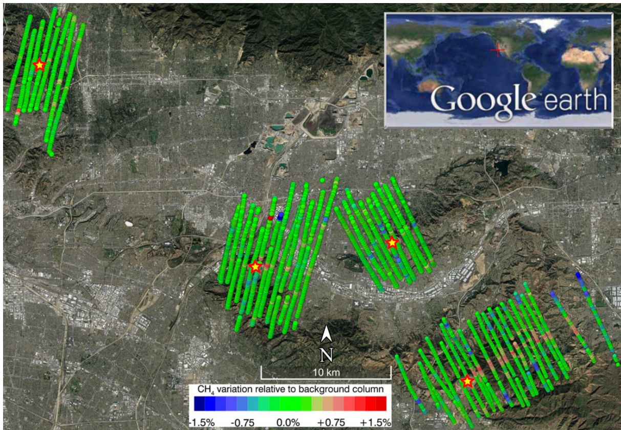
Figure 1. Shown are the MAMAP remote sensing survey flights over the four landfills (from left to right: the Scholl Canyon Landfill (SCL) on 27.08.2014, the Puente Hills Landfill (PHL) on 27.08.2017.2014, the BKK Corporation Landfill (BKK) on 01.09.2014 and the Olinda Alpha Landfill (OAL) on 01.09.2014) situated in the Los Angeles Basin (red cross in the world map, top right)in the main overview plot. Their-The locations of the landfills are marked by red/yellow stars. The MAMAP measurements are filtered by inclination to remove the turns and the colour code depicts \text{CH}_4 variations relative to the background (for details, see Sect. 3.1). Only the Olinda Alpha Landfill shows a clear plume in downwind direction. The wind direction was in general from south-west during the measurements. The map underneath is provided by Google Earth.
