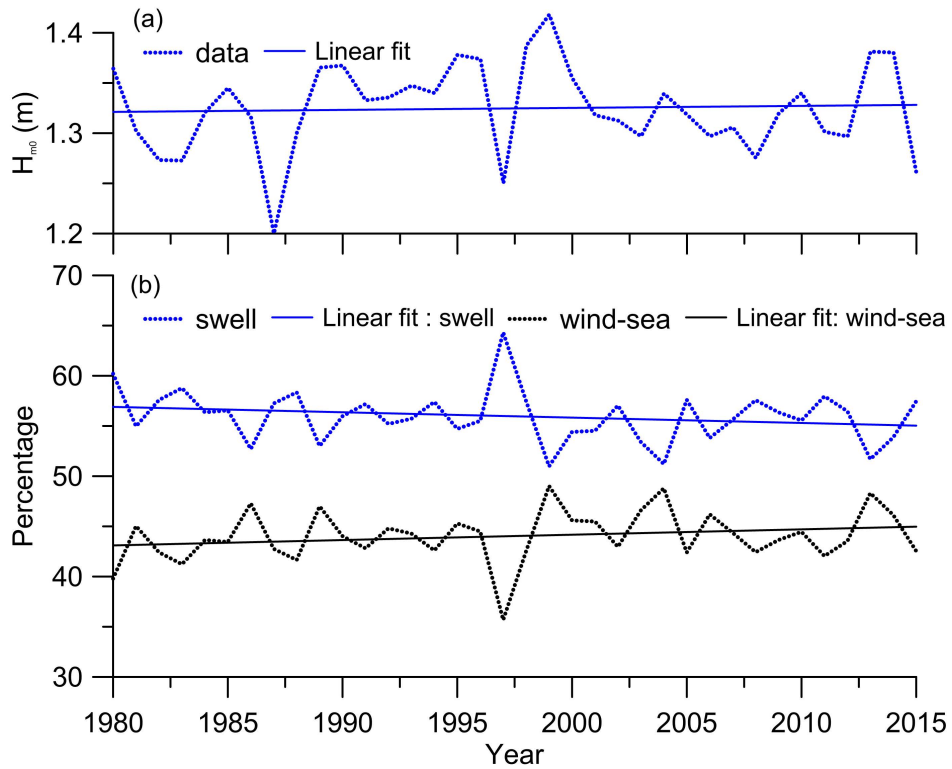
Fig. 2. Figure 11. Variation in a) significant wave height and b) percentage swell and wind-sea at 81°N; 78.29°E during 1980-2015. Linear trend is also presented
