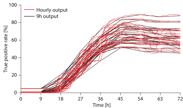
Fig. 4. Comparison of the ensemble prediction rates with 9h and hourly output time steps for the landslide-triggering rainfall events in August 2005 (a) and May 1999 (b).
