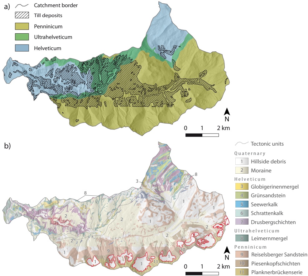
Fig. 3. Tectonic units with mapped extent of till deposits (a) and geological units (b) of the Laternser valley (Heissel et al. 1967, Oberhauser 1982).
