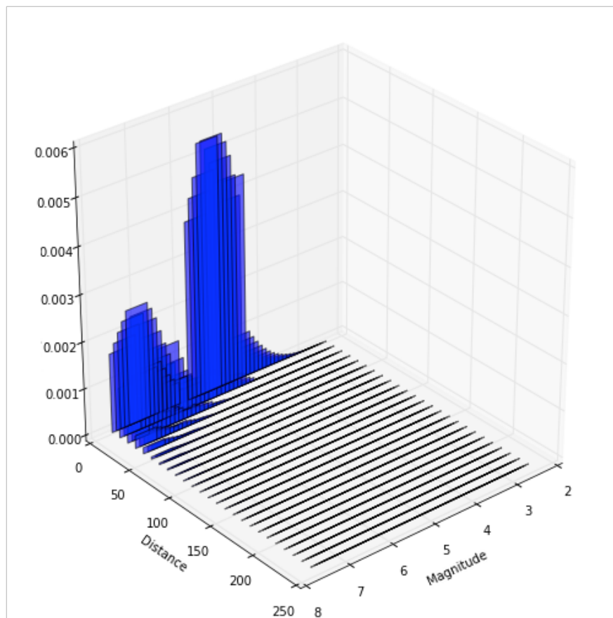
Fig. 2. Figure A: disaggregation plot (magnitude, distance, percentage) at 10% exceedence probability for exposure period of 30 years
