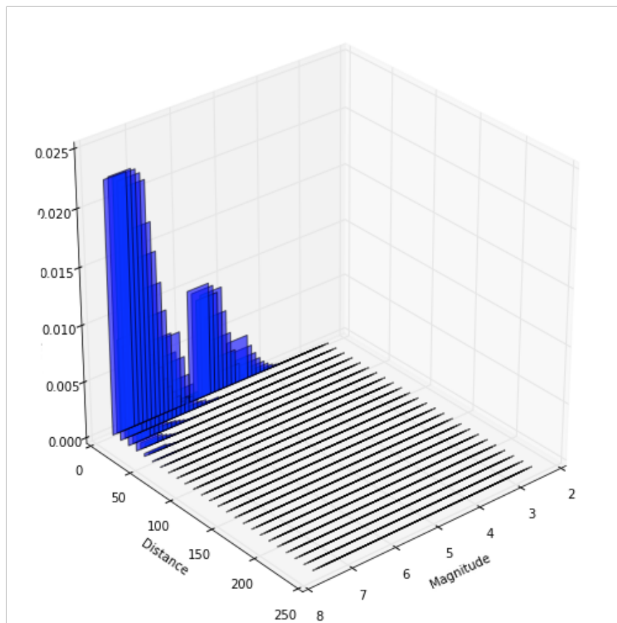
Fig. 4. Figure A: disaggregation plot (magnitude, distance, percentage) at 10% exceedence probability for exposure period of 1000 years
