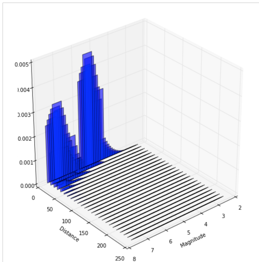
Fig. 3. Figure A: disaggregation plot (magnitude, distance, percentage) at 10% exceedence probability for exposure period of 50 years
