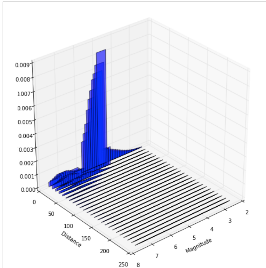
Fig. 1. Figure A: disaggregation plot (magnitude, distance, percentage) at 10% exceedence probability for exposure period of 5 years.
