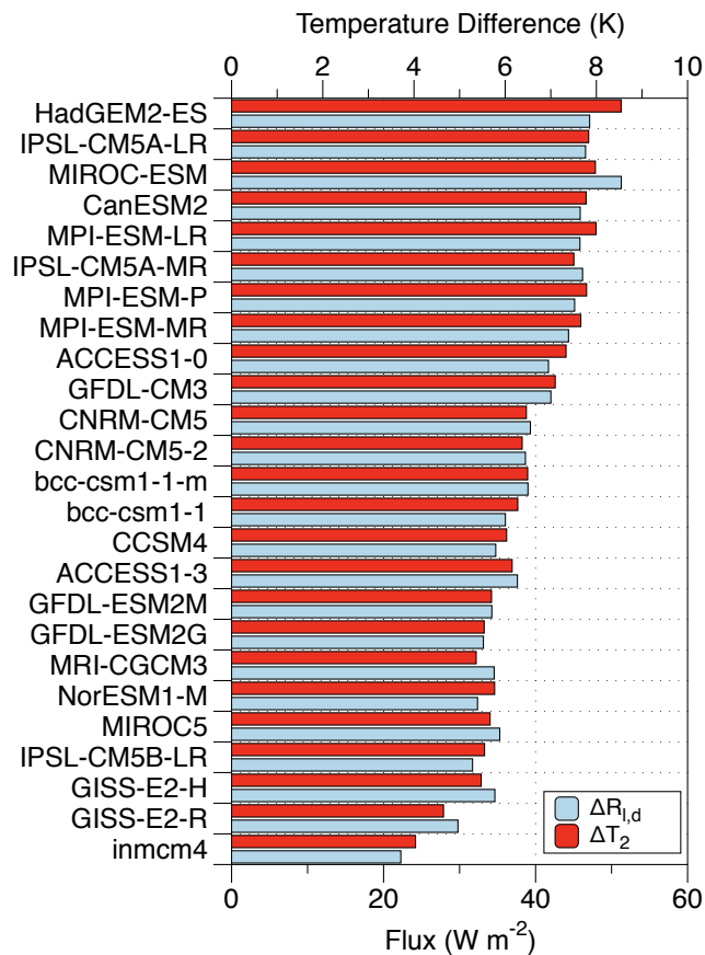
Fig. 1. Difference in downwelling longwave radiation ( \Delta R_{1,d} , blue) and near surface air temperature ( \Delta T_2 , red) between the 4xCO 2 scenario and the PreIndustrial (PI) control simulations of CMIP5.
