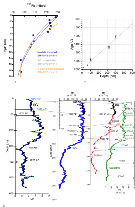
B Figure 1 Information used to construct our age model; A) ^{210}\text{Pb} activity downcore PO287-6B; B) MS correlation of PO287-6G to sedimentary sequences from the Tagus system (Abrantes et al. 2005); C) Depth vs. AD ages (with 2 \sigma error) for PO287-6G with a linear best fit.
