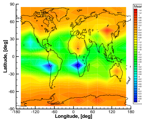
Figure 3. Deviation statistics obtained for real RO data: latitude-longitude map of inversion statistics of COSMIC observations relative to ECWMF profiles without fluctuations, for refractivity at altitude of 0.6 km. Results are shown for COSMIC events and concurrent ECWMF analysis fields from the 1st, 11th, and 21th day of every month of year 2008.
