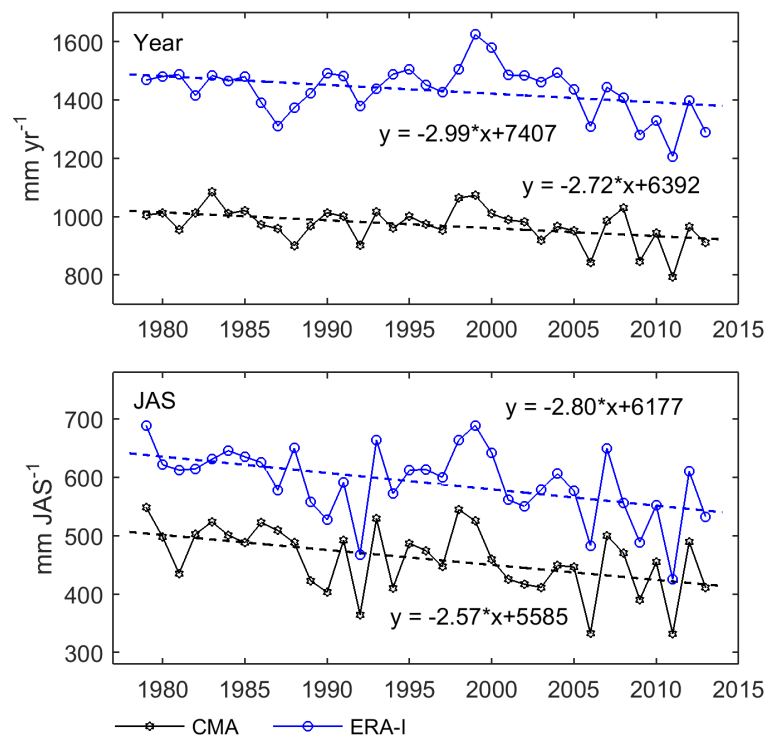
Fig. 3. The time series and trends of annual and summer (JAS) SWC precipitation
