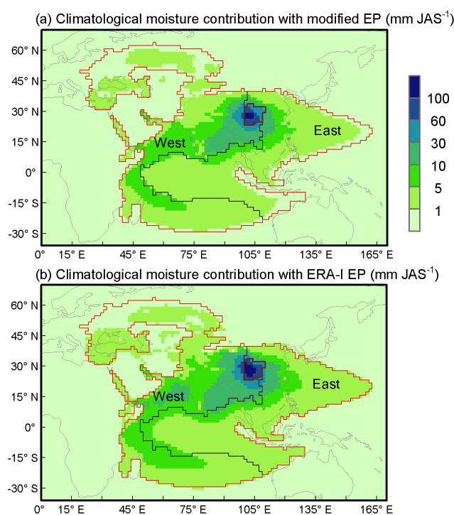
Fig. 1. Climatology of the summer moisture contribution
