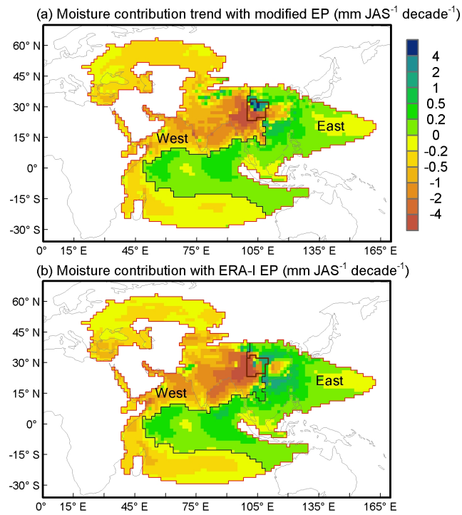
Fig. 2. The trend of the summer moisture contribution
